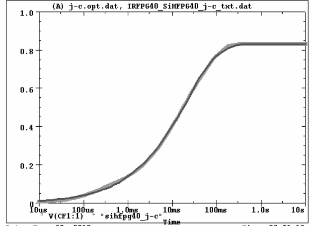
SiHFPG40 Filter j-c Temperature: 27.0
