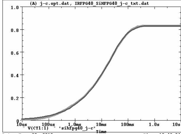
SiHFPG40 Tank j-c Temperature: 27.0
